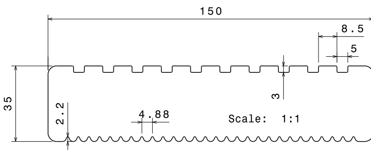
Figure 1: 150 x 35 DG Front View (mm).
