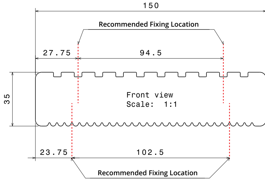
Figure 2: 150 x 35 DG Fixing Locations (mm).
