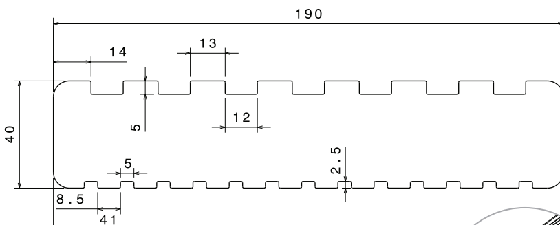
Figure 1: 190 x 40 DG Front View (mm).
