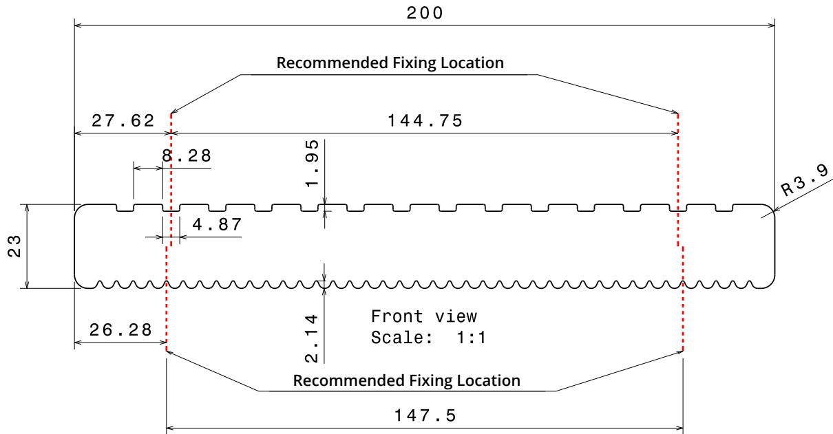
Figure 2: 200 x 23 DG Fixing Locations (mm).
