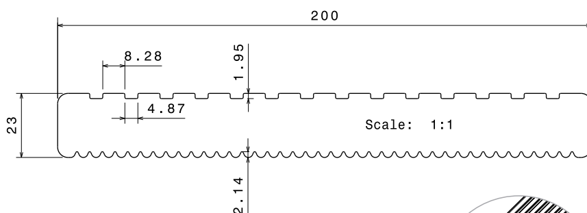
Figure 1: 200 x 23 DG Front View (mm).
